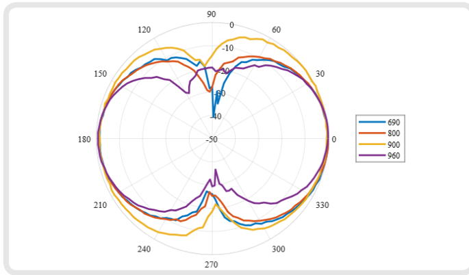
Azimuth: 690 - 960 MHz (top view)
