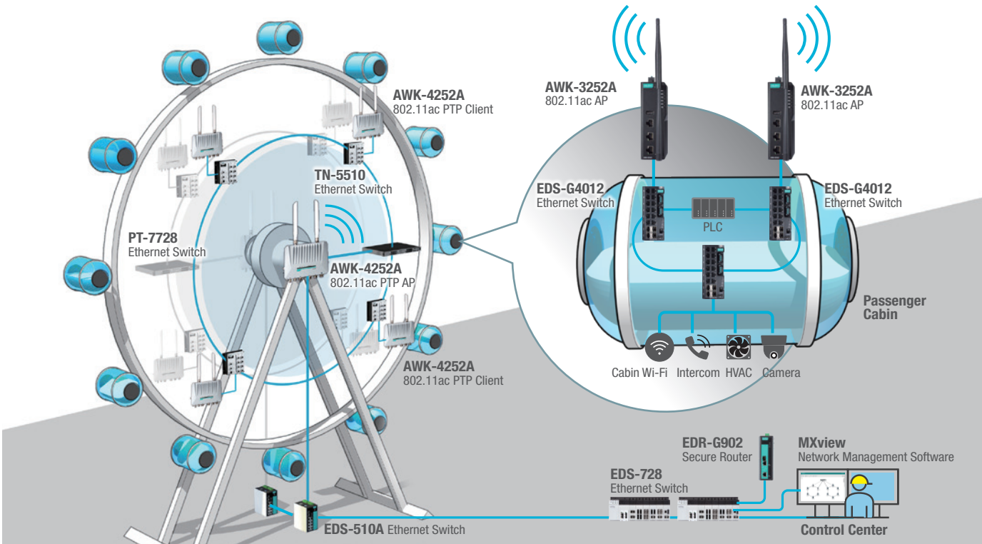
AWK-3252A 802.11ac Wireless AP/Client
