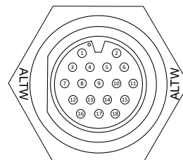
X-Lock Amphenol (Socket)
